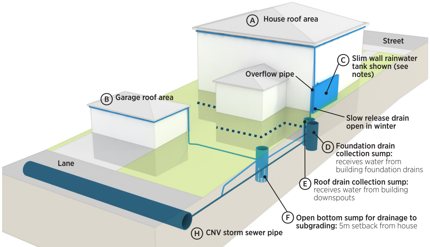
PERSPECTIVE VIEW
