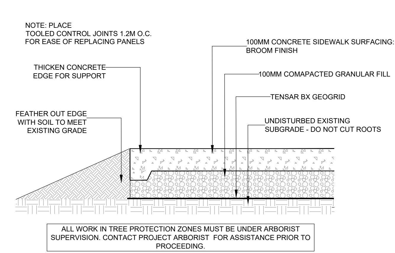
3 SIDEWALK DETAIL THROUGH ROOT ZONE 1:10
