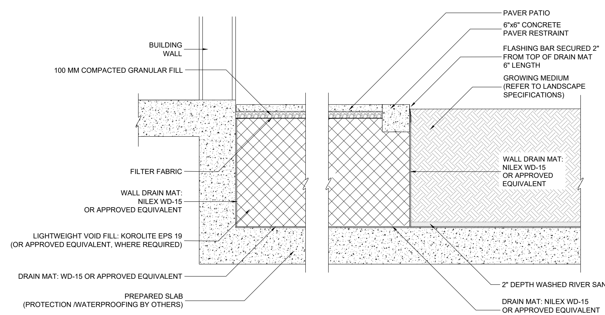
6 PATIO/LANDSCAPE AT SLAB DROP 1:25
