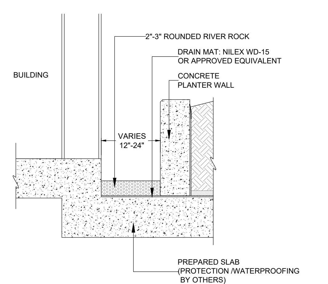
2 DRAIN ROCK STRIP AT BUILDING ON SLAB 1:25
