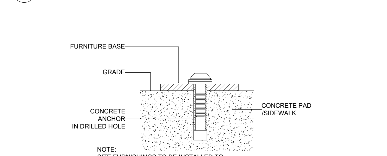
10 SITE FURNITURE MOUNTING N.T.S
