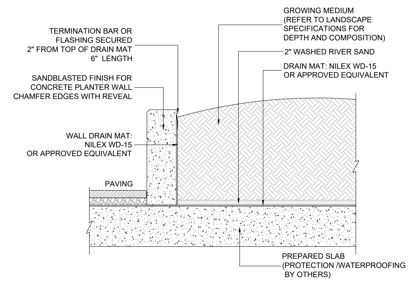
4 PLANTER WALL ON SLAB 1:25
