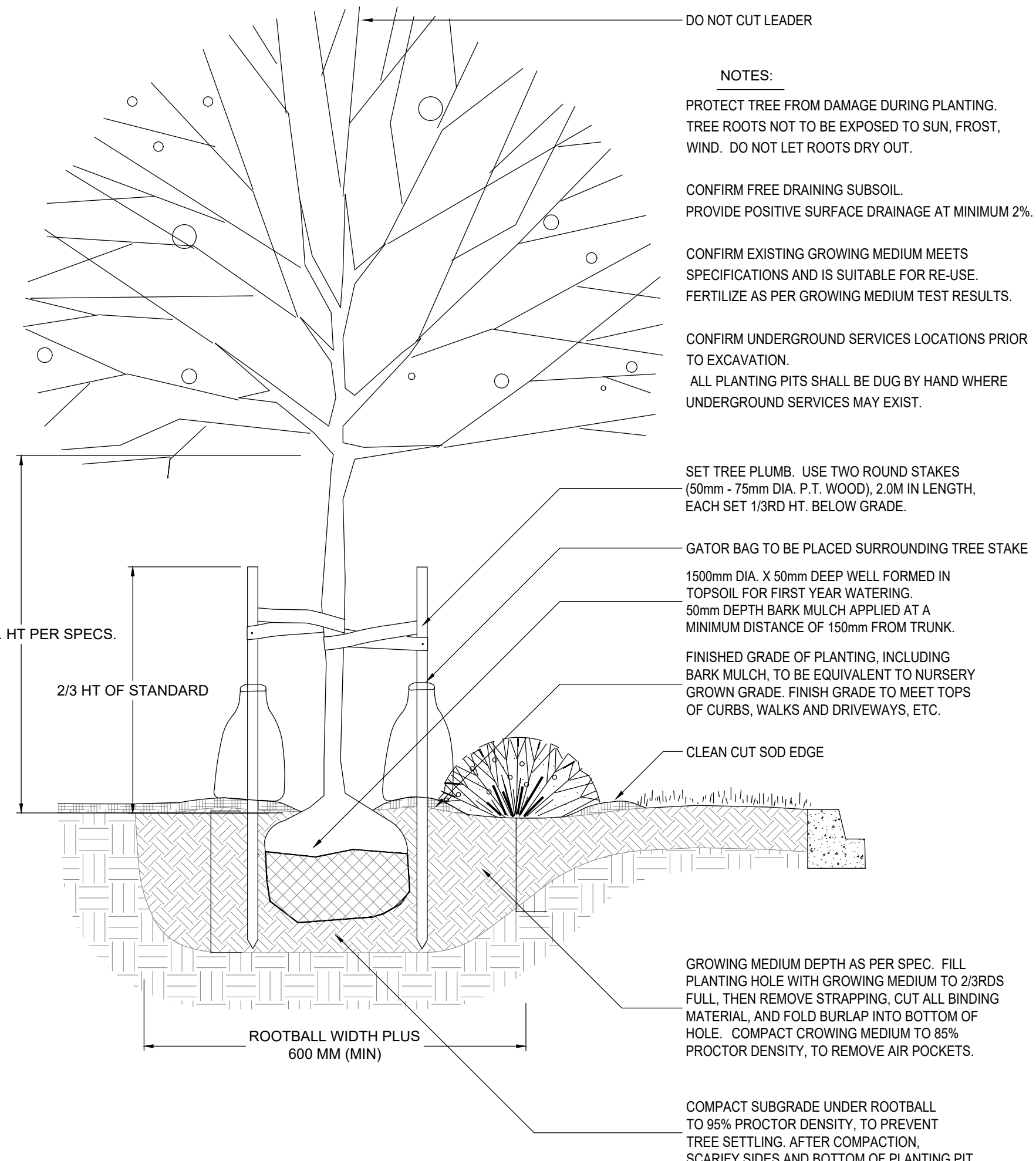
5 TREE AND SHRUB PLANTING AT GRADE 1:25
